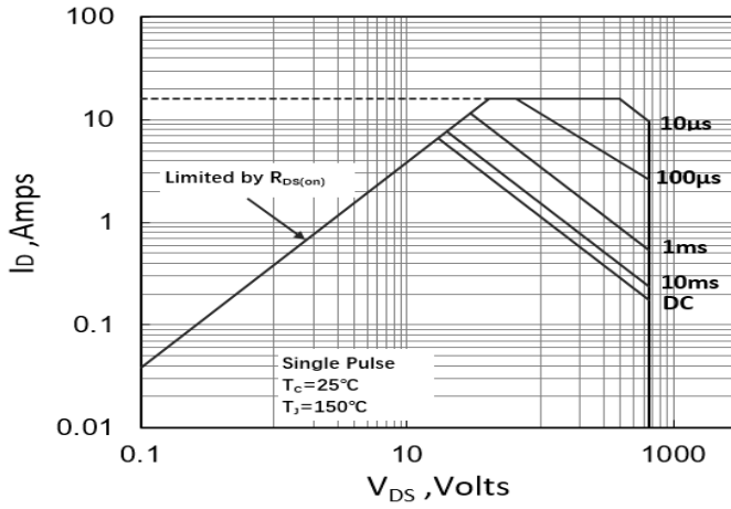
Figure 13. Maximum Safe Operating Area (TO-252/TO-251)
