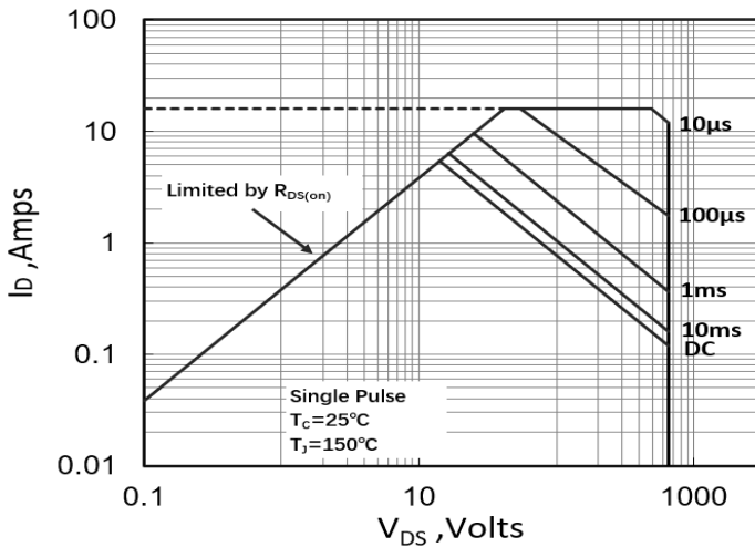
Figure 9. Maximum Safe Operating Area (TO-220)
