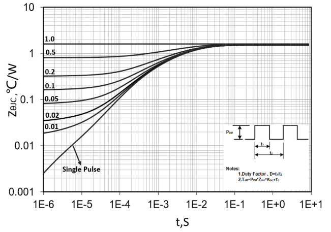
Figure 14. Transient Thermal Response Curve (TO-252/TO-251)
