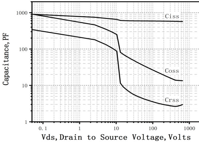
Figure 7. Capacitance Characteristics
