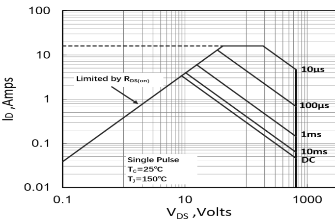
Figure 11. Maximum Safe Operating Area (TO-220F)
